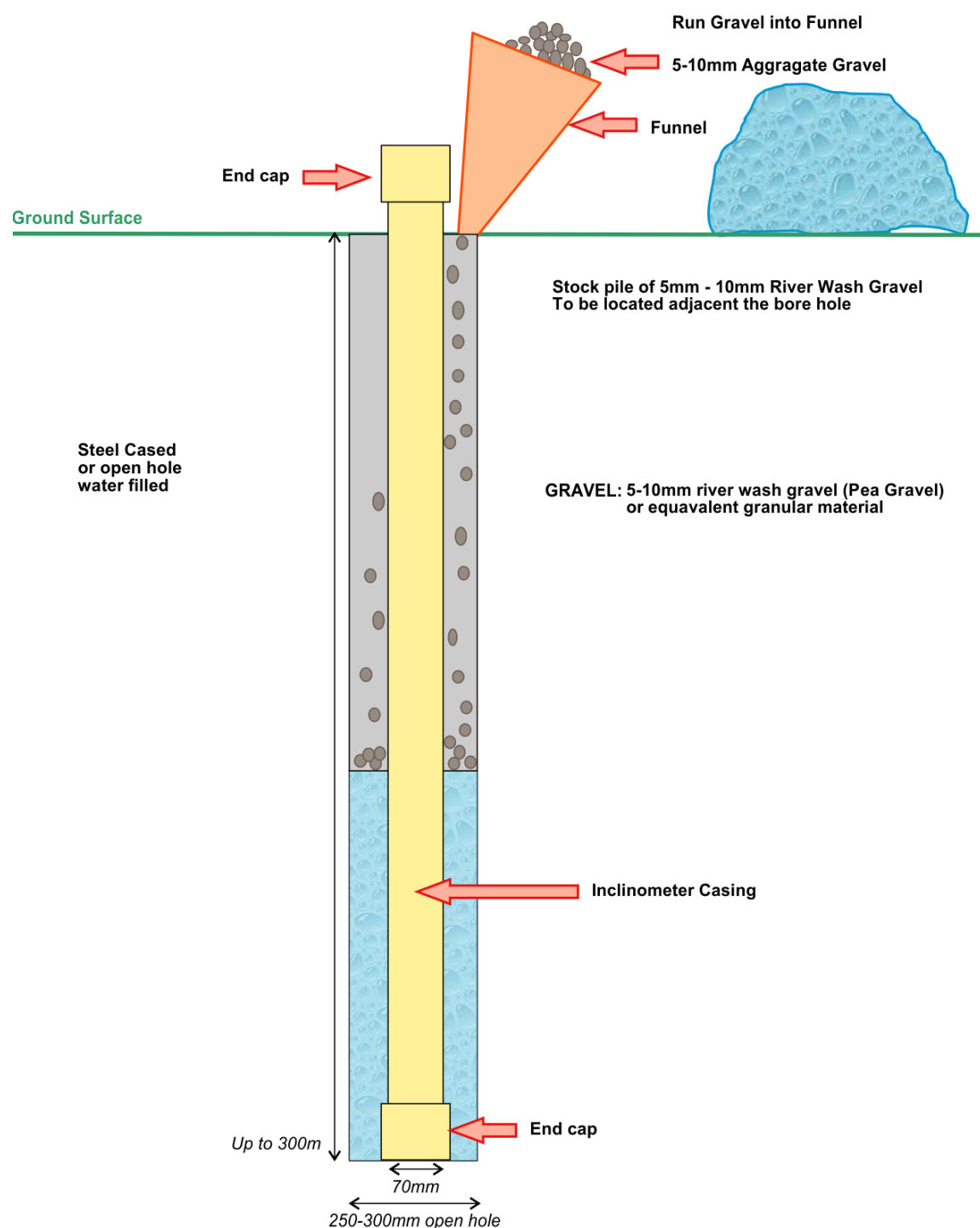
Figure 6: Schematic of typical inclinometer casing installation used by SCT.
