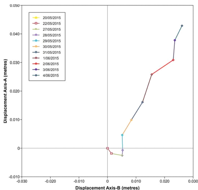
Figure 9: Vectors plot: 207.5 meters
