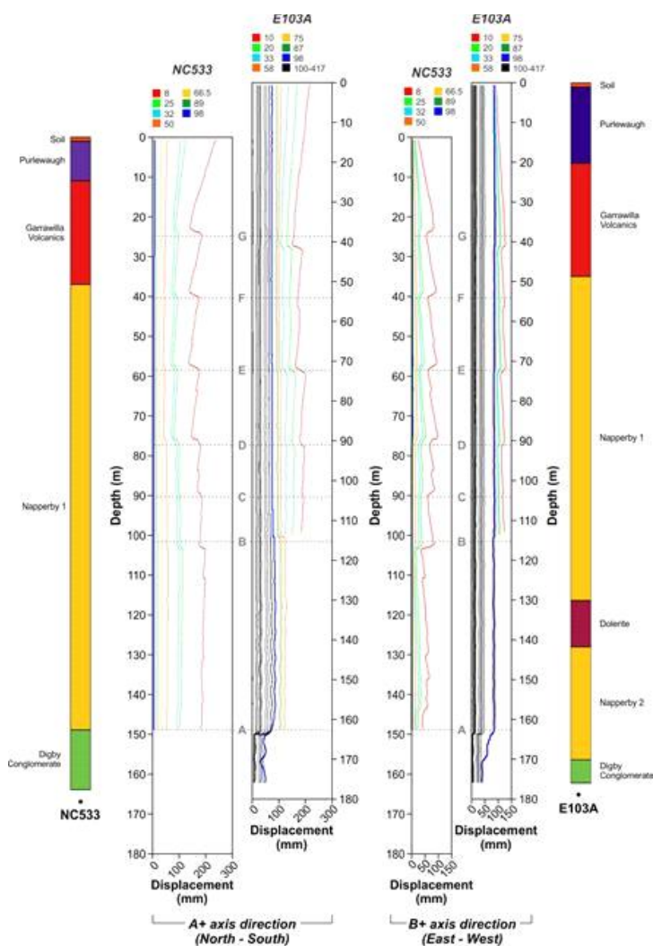
Figure 11: Inclinometer movements measured in the A+ (North - South) and B+ (East - West) axis directions (after Mills et al. 2015)
