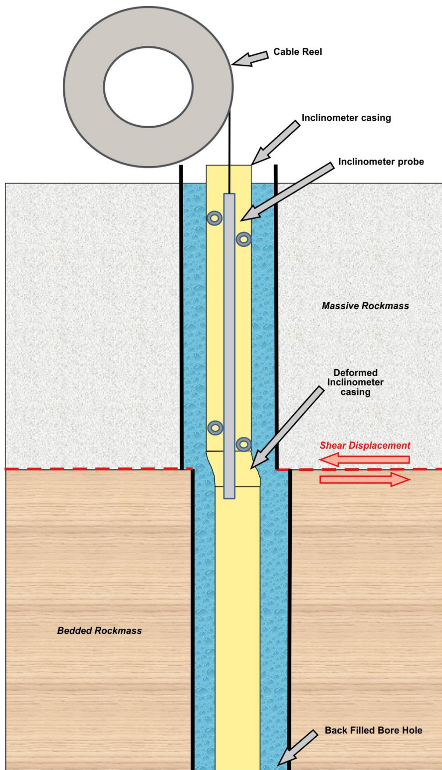
Figure 5: Schematic view of Inclinator casing and Inclinator probe.
