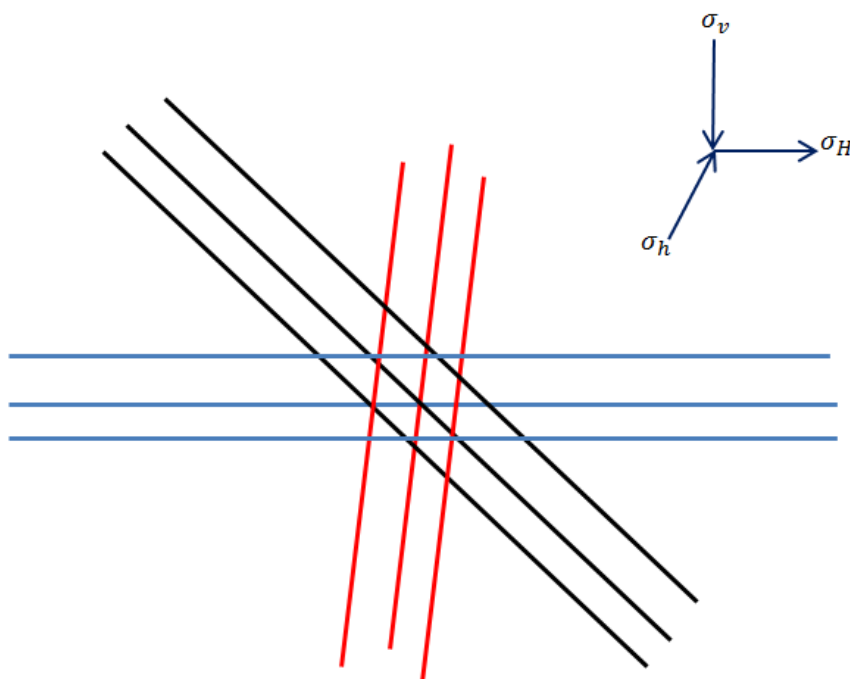
Figure 3: Approximate acting stress on each discontinuity set as a function of field stress orientation and orientation that discontinuity set
